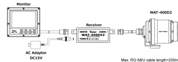
Max. RG-58/U cable length=200m
